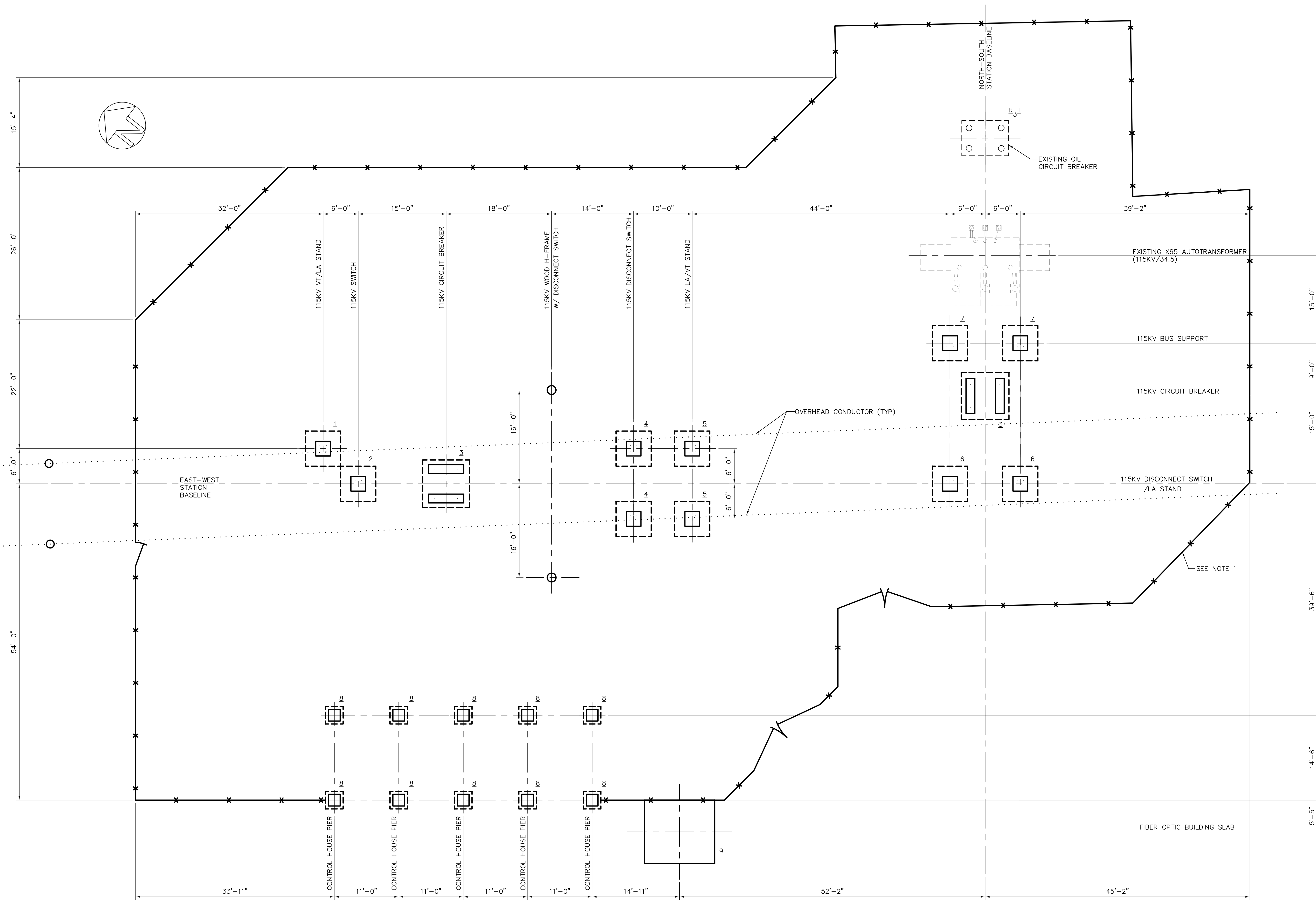
FOUNDATION PLAN SCALE: 1/8"=1'-0"
